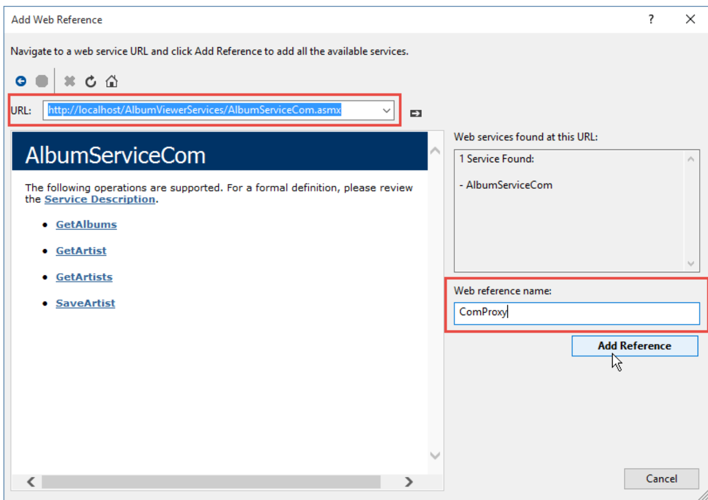
Figure 17 – Adding a second service with a new service reference/namespace. The new namespace will be completely separate from the original service imported even if type names overlap (ie. both services have an Artist class: Proxy.Artist and ComProxy.Artist which are different in the eyes of .NET even though they have the same signature)
